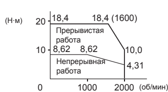
R88M-G90010T (900 Вт)
